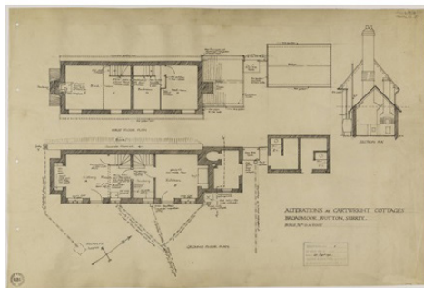
Design for alterations to Cartwrights, 1911
